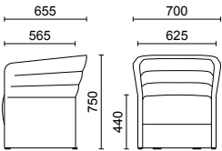
SINGLE-SEATER, BASE WITH 4 LEGS IN TAPERED TUBULAR STEEL
