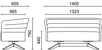
2-SEATER, SWIVELLING, WITH 4-STAR BASE IN TUBULAR STEEL, SWIVELLING TABLET WITH SWIVELLING SUPPORT
