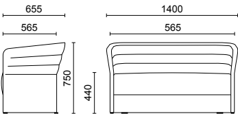
2-SEATER WITH FLOOR-STANDING BASE
