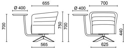
1 SWIVEL SEATER WITH CENTRAL ROUND STEEL BASE
