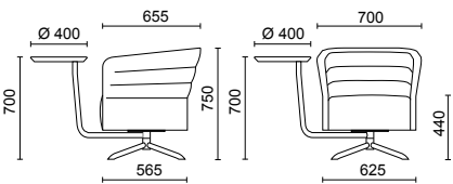
SINGLE-SEATER, SWIVELLING, 4-STAR BASE IN WOOD
