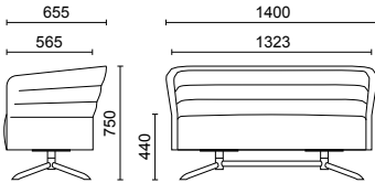
2-SEATER, 4-STAR BASE IN WOOD, DOUBLE SWIVELLING TABLET WITH SWIVELLING SUPPORT
