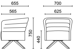
SINGLE-SEATER, SWIVELLING, BASE WITH 4 LEGS IN TAPERED TUBULAR STEEL
